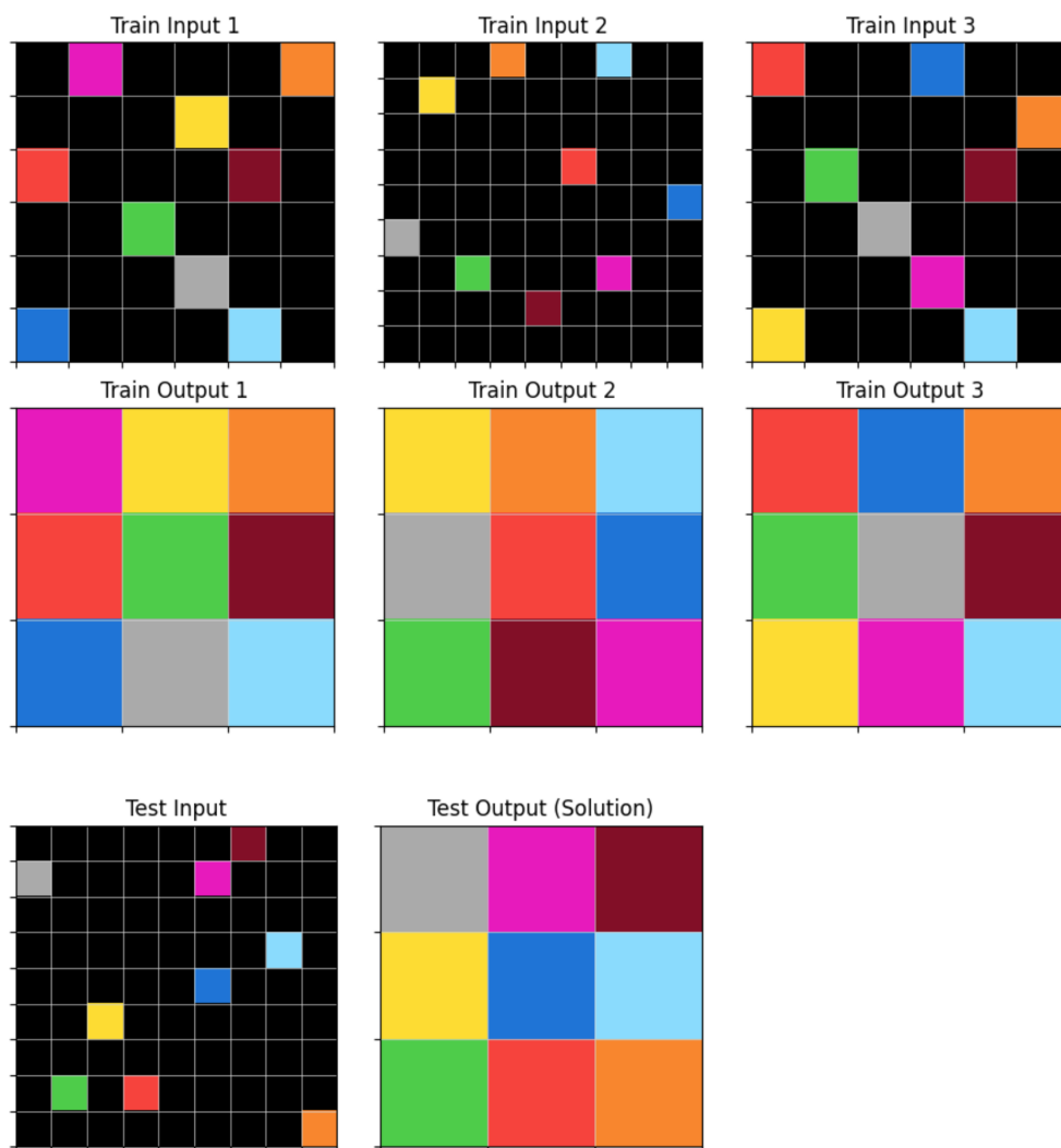
Figure 13: LPN Example 3
